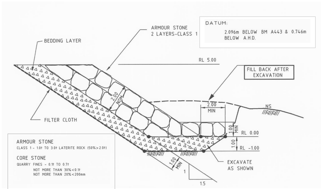
Figure 56: Emu Point Foreshore stabilisation revetment typical cross-section, May 2007 (Source: DoT, DWG 452-12-2)
