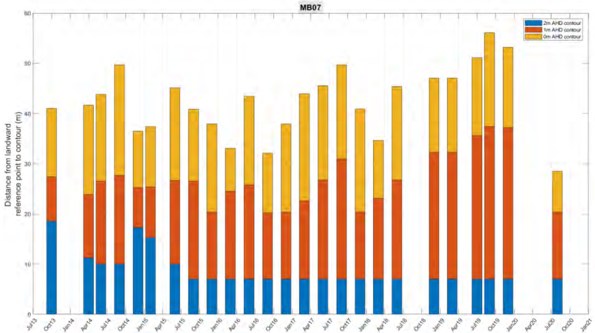
Figure 51: Seaward location of different aerial beach contours (0m, 1m, 2m AHD ) from a static landward control point along beach transect MB-07.
