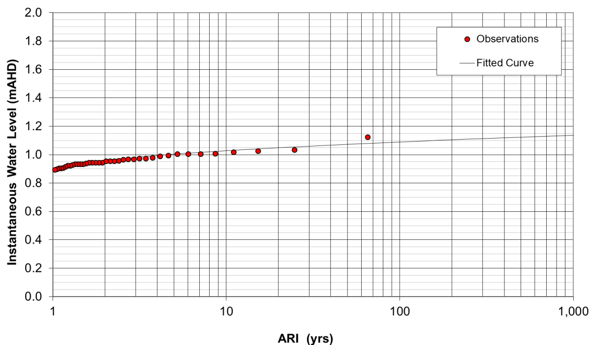
Figure 3.18 Extreme Water Level Analysis for Albany (MRA, 2018)
